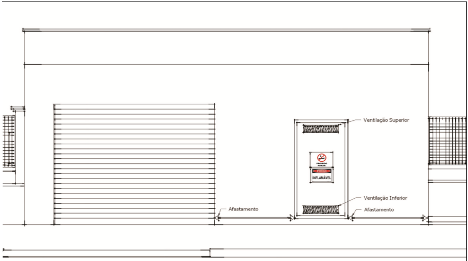
Figura 03: Central de GLP – “nicho”
